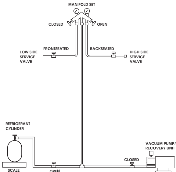
CHARGING CONNECTIONS
